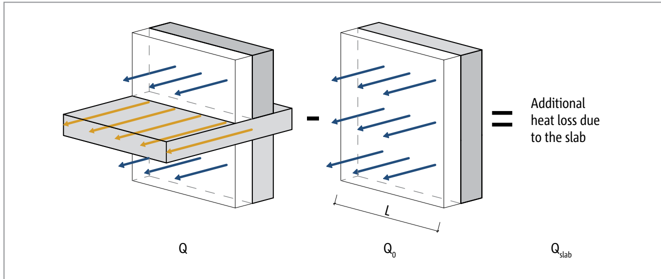
Figure 2: Example of process of determining the linear transmittance of a slab penetrating a wall
