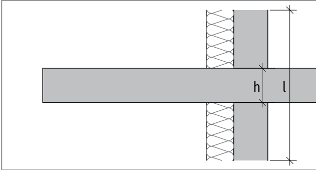
Figure 3: Assembly 1 – Balcony with thermal bridge
