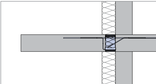
Figure 4: Assembly 2 – Balcony with thermal break element
