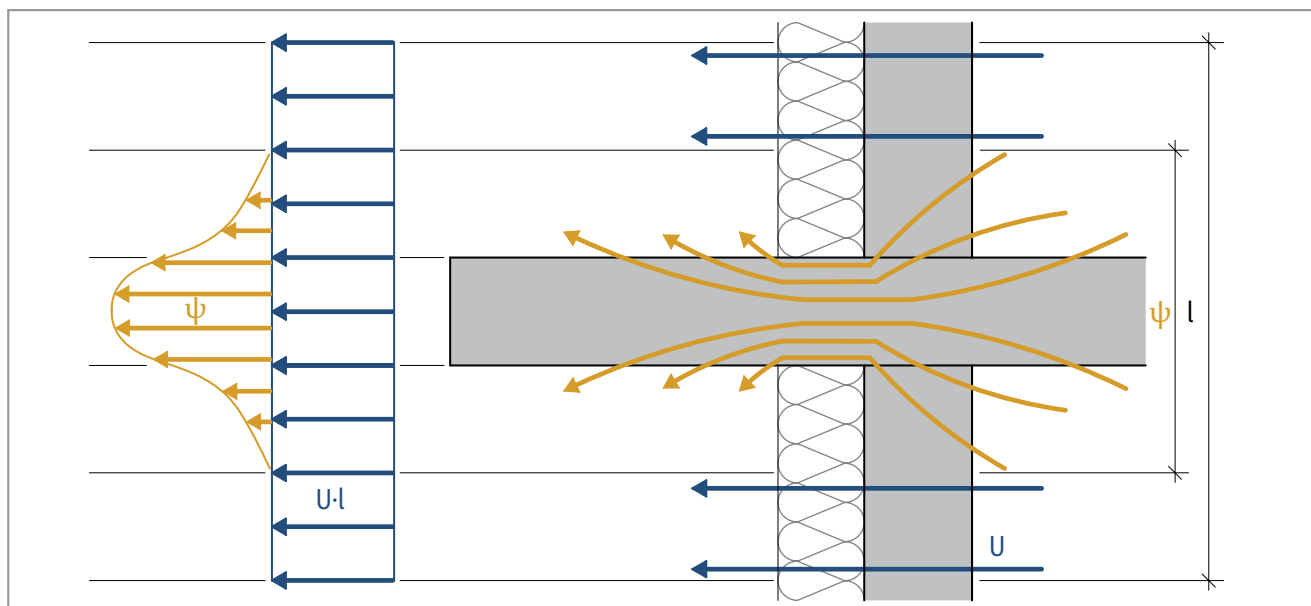
Figure 1: Pattern of heat flow through a building enclosure with materials that allow lateral heat flow to a thermal bridge
